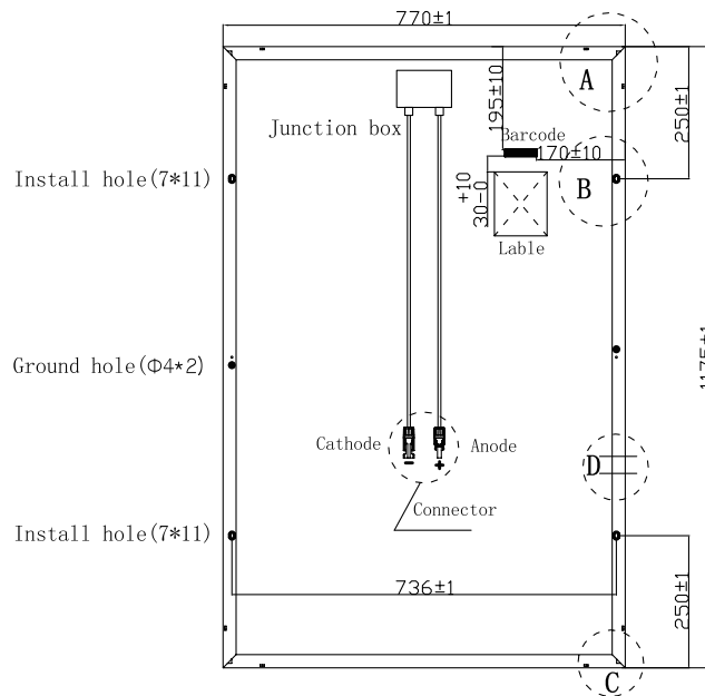
Install hole (7*11)
