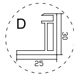
Frame cross-section
